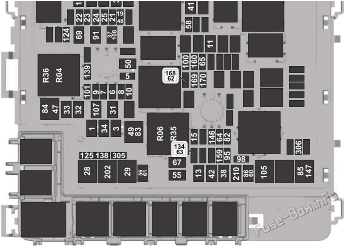
Assignment of the fuses in the engine compartment (2021, 2022)
